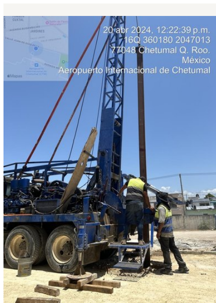
Drilling with truck-mounted equipment.
