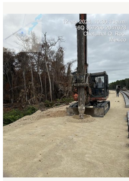
Drilling with crawler-mounted equipment.
